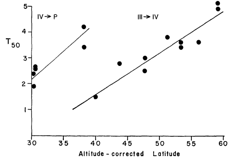
FIG. 9. Depth of diapause as measured by T_{50} , the number of pulsed long days required to terminate diapause in 50% of the sample. T_{50} 's for the termination of III instar diapause were used to calculate the altitude:latitude conversion factor, 49m: ^\circ\text{N} (Eqs. 6-7), which was then used to correct for altitude of IV instar diapausing populations. Actual T_{50} 's and sample sizes are given in Appendix I.
